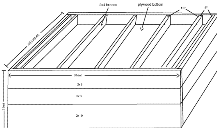
Figure 4. Top section of planter shown upside down to view construction. The first 2x4 brace is placed directly against the outside piece. The second bottom brace on either side is in 6 inches, then the remaining three braces are 13 inches apart. Drill holes at one-foot intervals before turning over.
