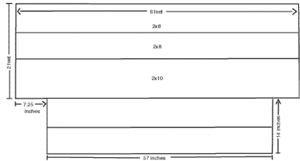
Figure 2. Side view of tall planter.
