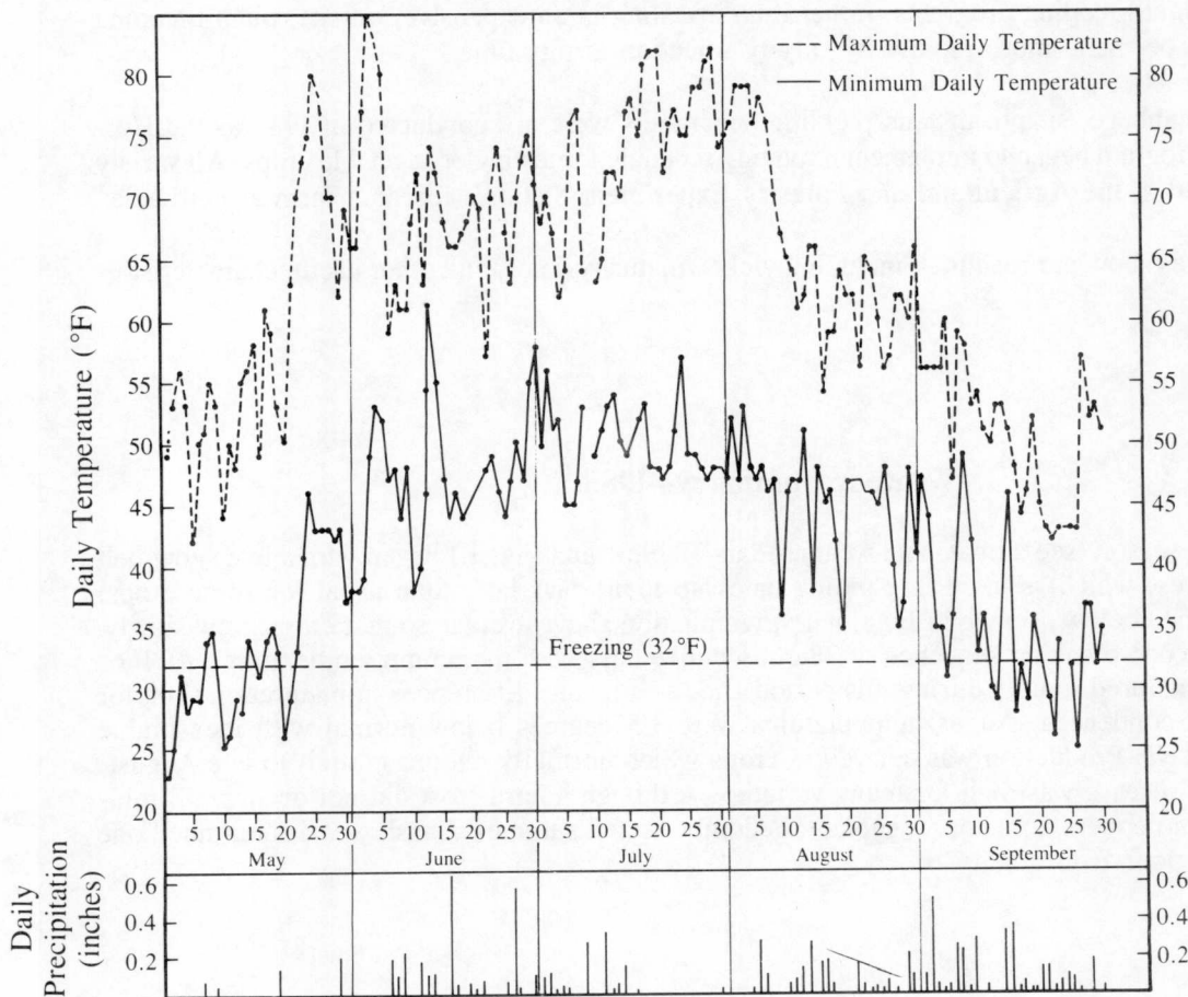
Figure 1. Daily weather data, May through September, 1985, University of Alaska-Fairbanks, Agricultural and Forestry Experiment Station.
