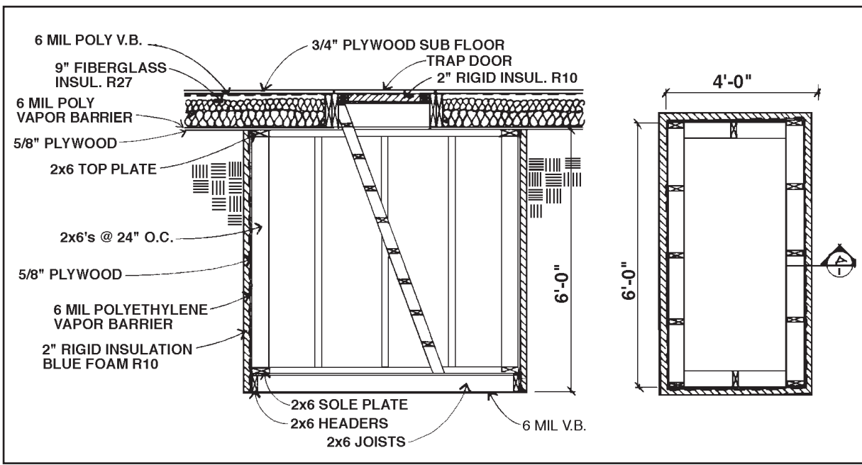
Figure 1. Example of a blueprint for below-floor root cellar
